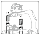
俯仰轴延长模块 60 mm
